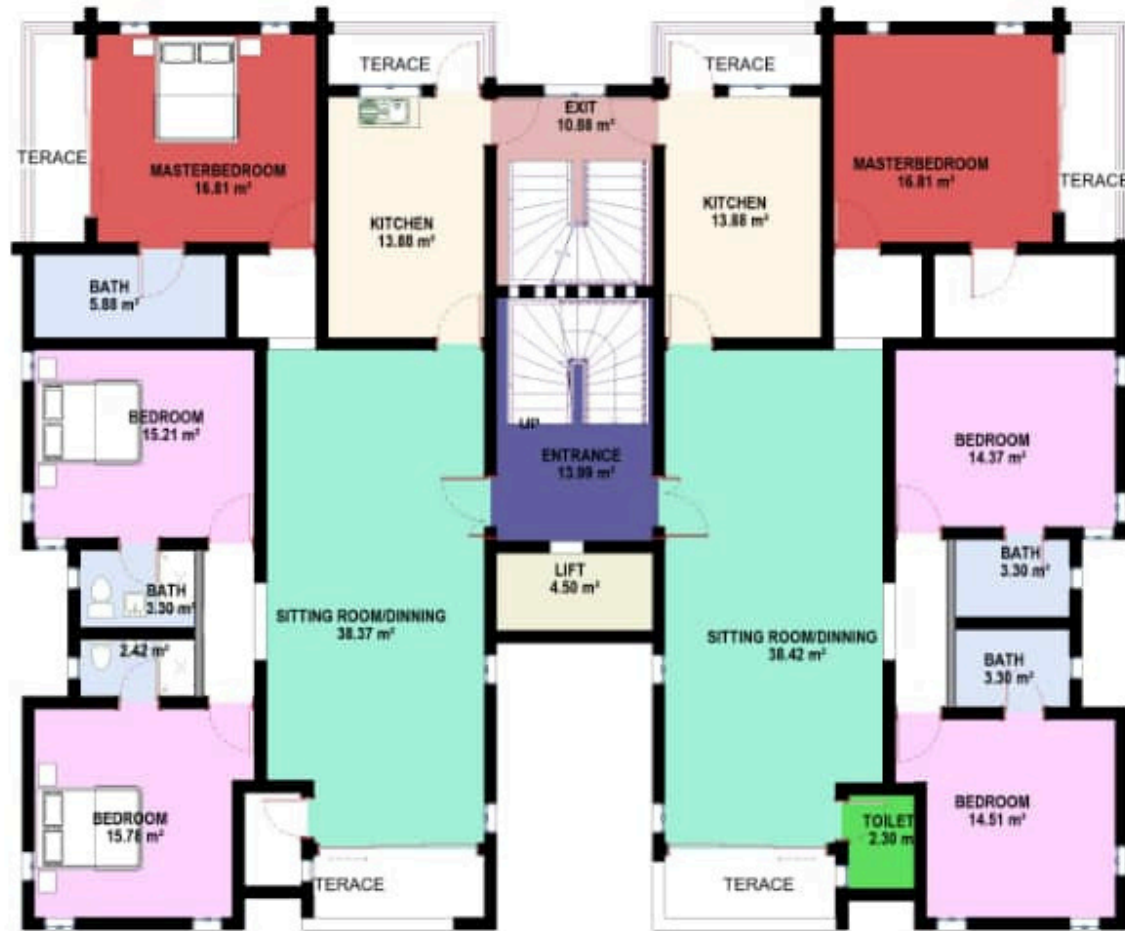
1 st & 2 nd FLOOR PLAN
